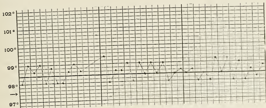
Fig. 240.—Temperature in an early case with lesion at right apex.
